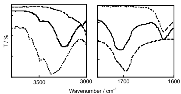
Fig. IR spectra of a ground mixture of 1a and 2-methylglutaric acid (solid line), 1a (dotted line), and 2-methylglutaric acid (dashed line) in a Nujol mull.
