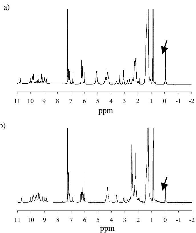
Fig. ^1\text{H} NMR spectra ( \text{CDCl}_3 ) of a) the authentic complex of 1a and methyl- \beta -D-glucopyranoside and b) a ground mixture of 1a and methyl- \beta -D-glucopyranoside. The arrows indicate the upfield shifted methyl resonance of the glycoside.
